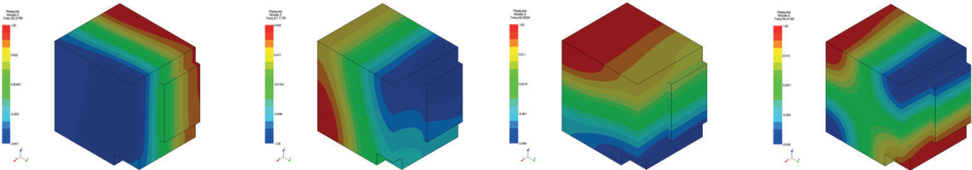
Illustration of room modes ( acoustic phase contours )
