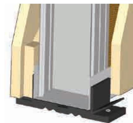
Vibro-WS support systems for a floating gypsum board partition
